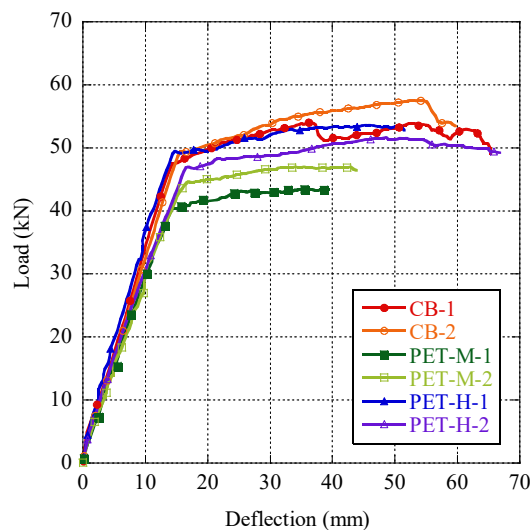
Fig. 10. Load-Deflection of the beams.
