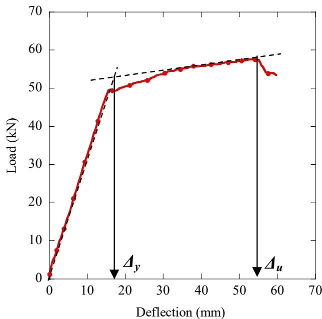
Fig. 16. The calculation method of ductility index.
