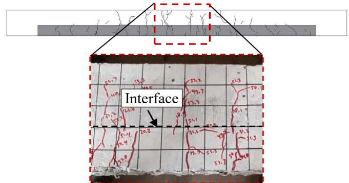
Fig. 14. Concrete interface at PET hybrid beam.
