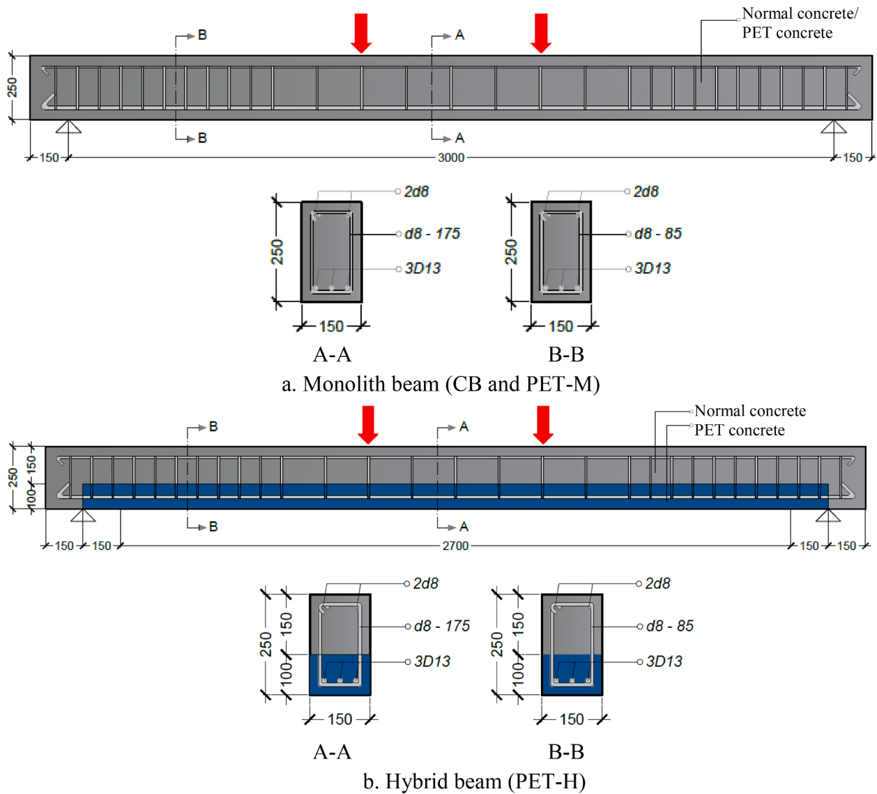
Fig. 4. Details of specimens.
