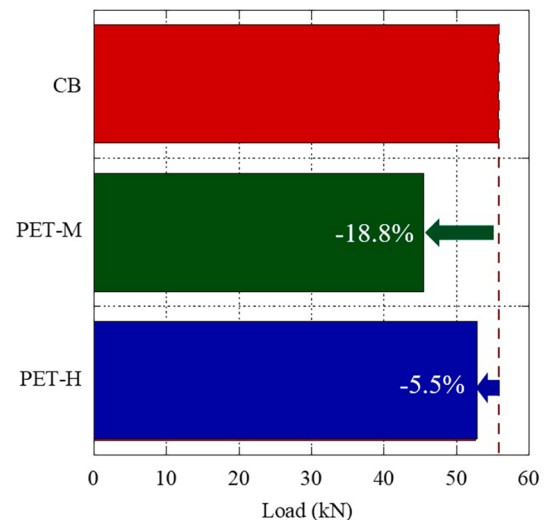
Fig. 11. Strength reduction.
