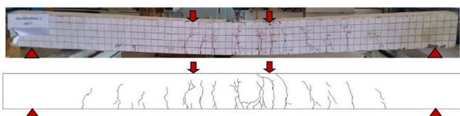
Fig. 12. Crack pattern of CB.
