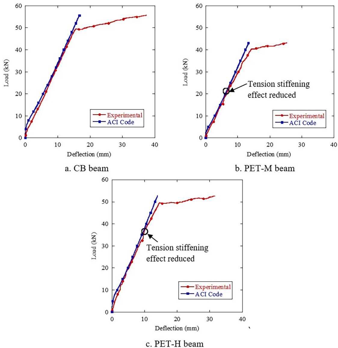
Fig. 17. Comparison between the measured and calculated deflections.
