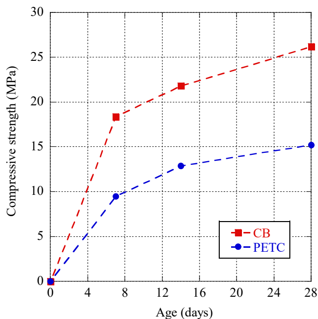
Fig. 7. Compressive strength.
