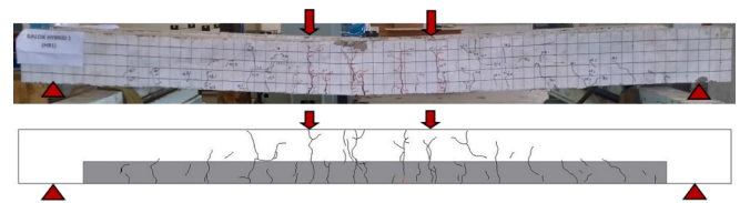
Fig. 13. Crack pattern of PET-H.
