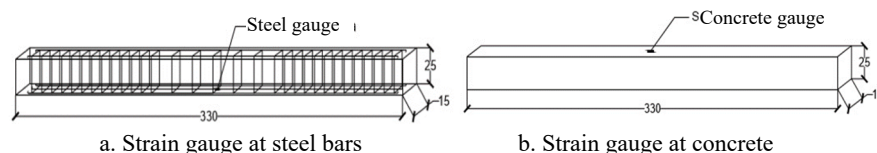
Fig. 5. Location of strain gauge.
