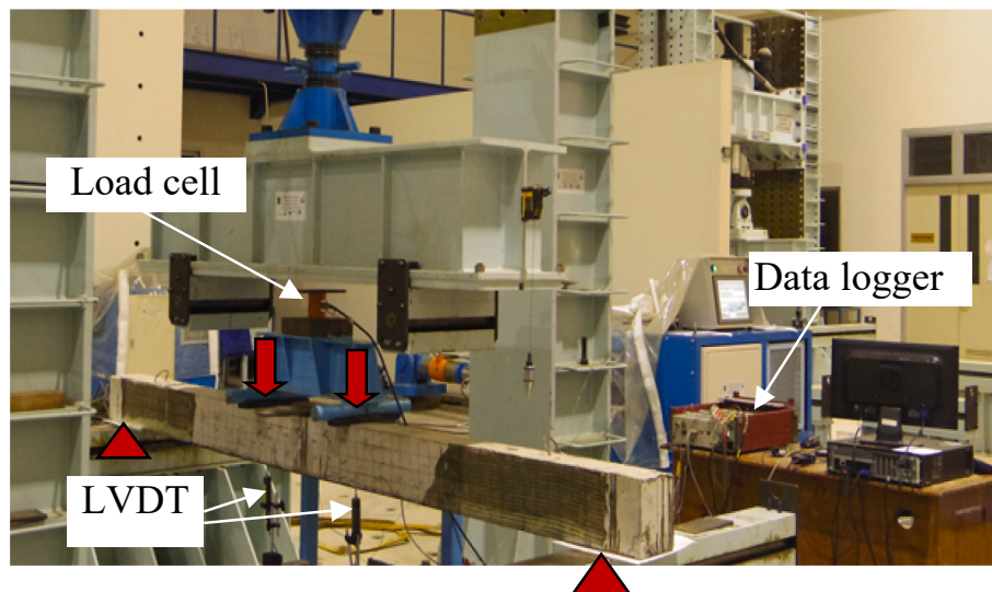
Fig. 6. Loading test.
