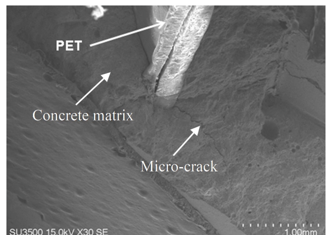
Fig. 8. SEM test of PET waste concrete.
